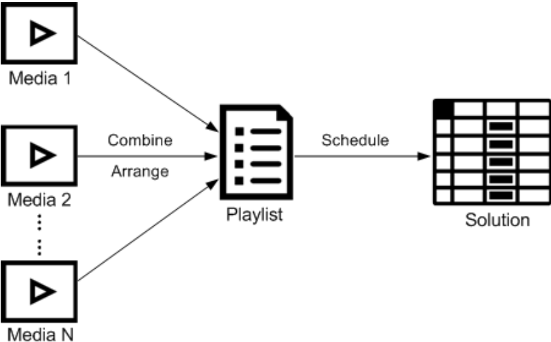
Figure 1-1 Media management
