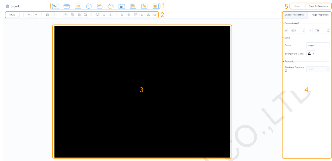
Figure 4-1 Editing page
