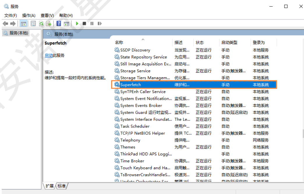
图4-8 Superfetch
