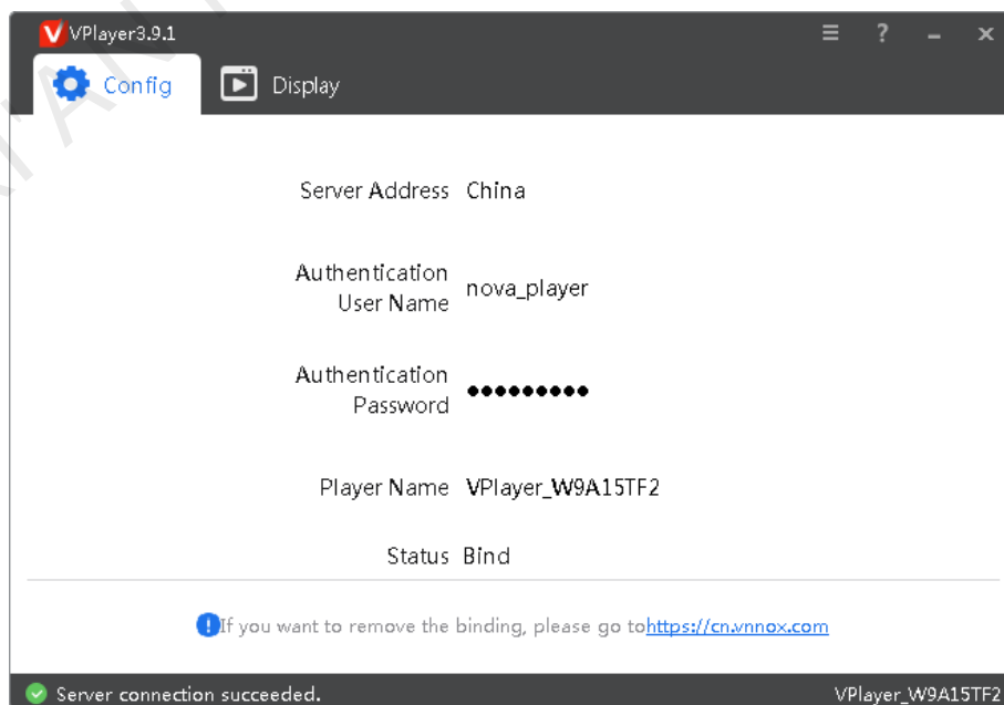
Figure 3-4 Binding successful
