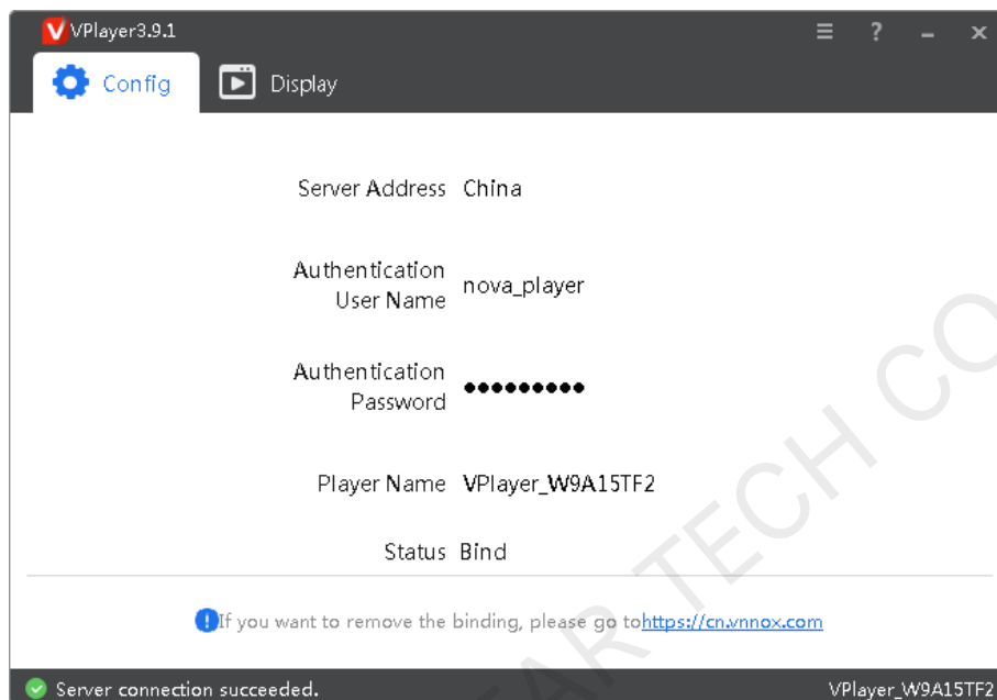
Figure 3-3 Authentication information
