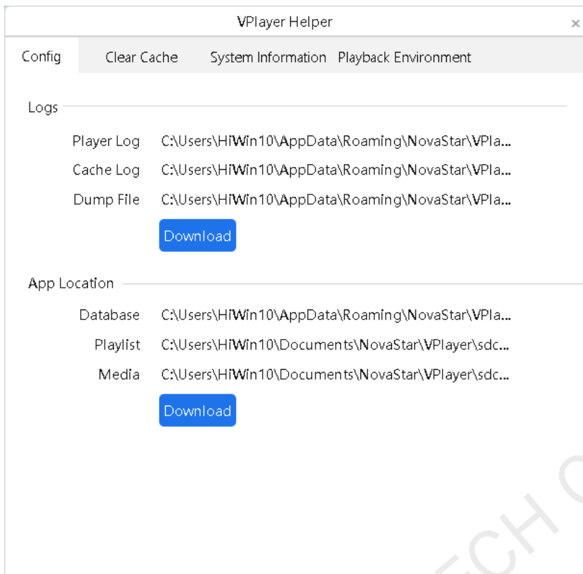
Figure 5-2 VPlayer Helper
