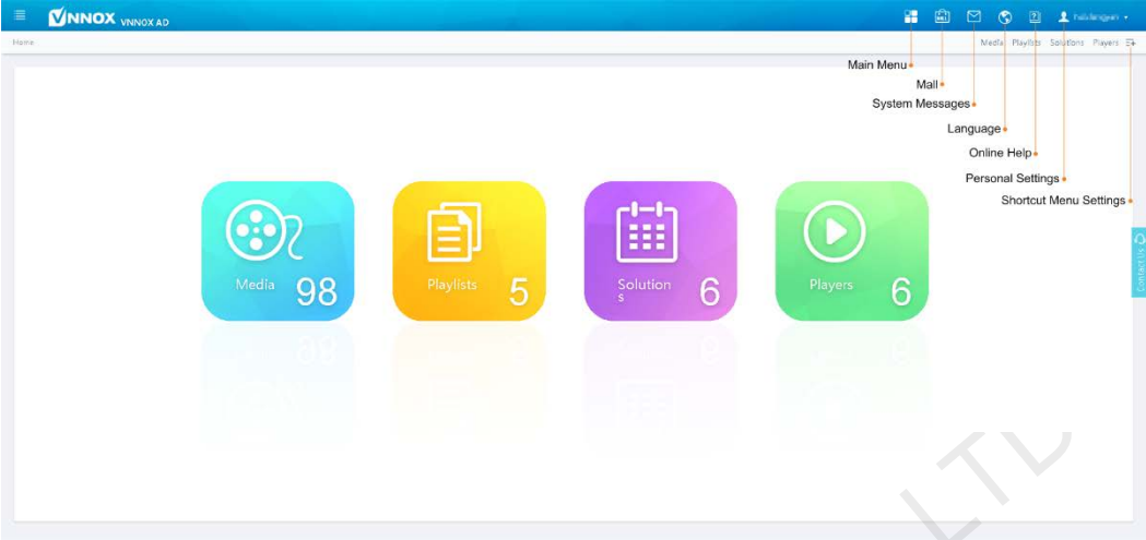
Figure 3-2 VNNOX AD
