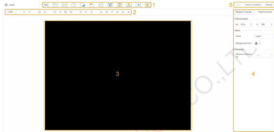
Figure 4-1 Editing page
