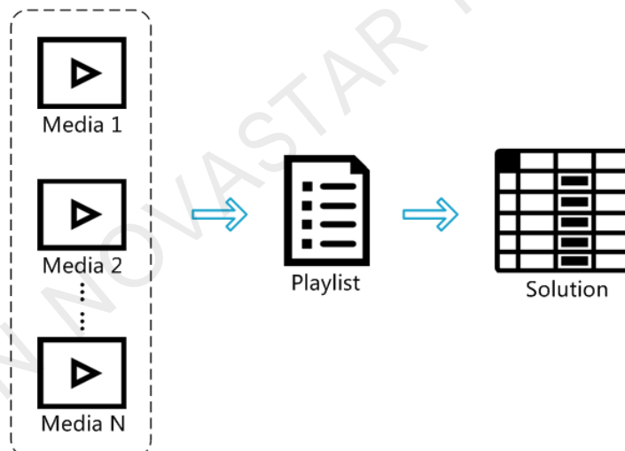
Figure 1-1 Media management
